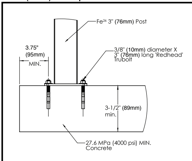
Fe 26 3" (76mm) Post Top Mount To Concrete
