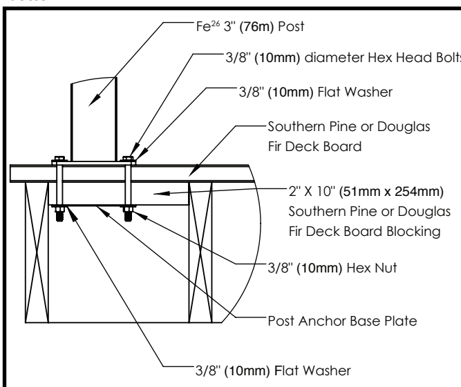
Fe 26 3" (76mm) Post Top Mount To Southern Pine or Douglas Fir Floor Joist Mounted Perpendicular
