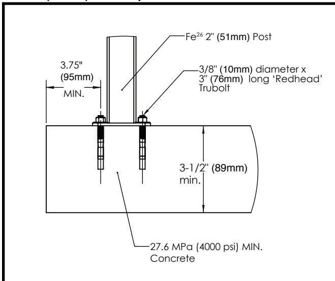
Fe 26 2" (51mm) Post Top Mount To Concrete
