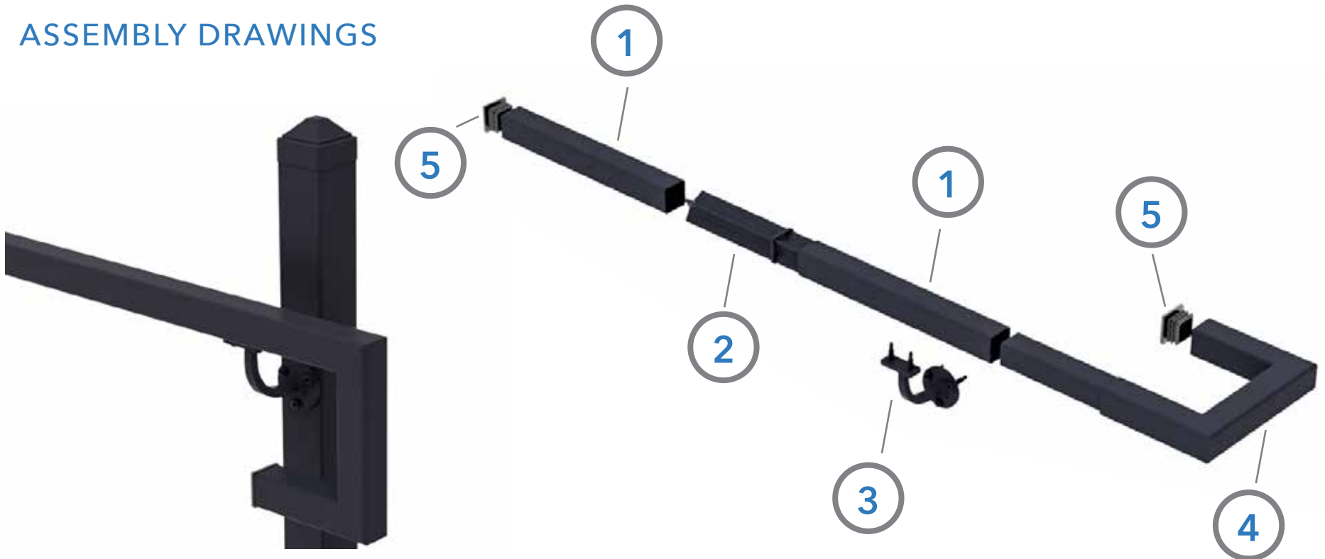
HR-RETURN HR-Ext 4.5" x 7" (125mm x 178mm)
