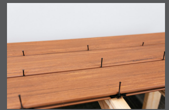
CLIP IS NOW FIRMLY IN PLACE NO PRE-INSTALL IS REQUIRED
