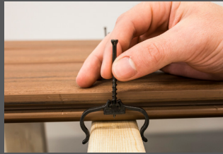
SIMPLY ATTACH CLIP LEGS AROUND JOIST
