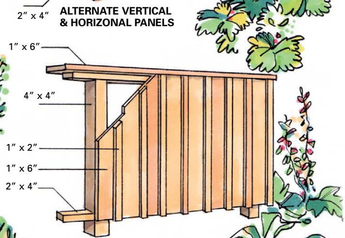
VERTICAL BOARD-AND-BATTEN
